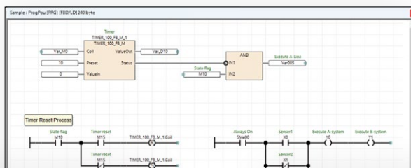
Function block diagram (FBD)
